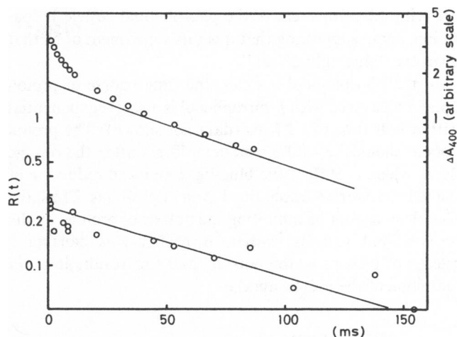
FIGURE 4 Time course of decay of the M intermediate (upper curve) and of the reduction in proton pumping caused by blue light (lower curve) in reconstituted phospholipid vesicles. Egg phosphatidylcholine vesicles, the characteristics of which are described in Fig. 2 were used here. The pH of the sample was maintained at 6.8 \pm 0.1 . Other conditions and definitions are the same as in the legend of Fig. 3.
