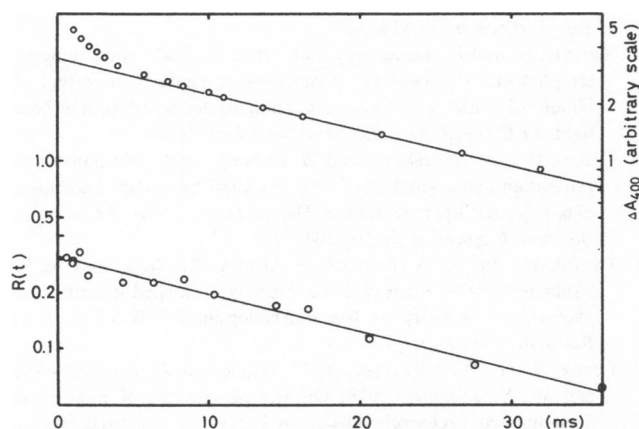
FIGURE 3 Time course of the decay of the M intermediate (upper curve) and of the reduction in proton pumping caused by blue light (lower curve) in cell envelope vesicles. The decay kinetics of M intermediate were measured as described by Govindjee et al. (15) except that the actinic light source was replaced by the 200 \mu\text{s} flash used for the glass electrode experiment. The delay time between the orange and the blue flashes was varied and signal from the electrode following the double excitation was recorded. The amplitude of pH change was obtained by extrapolating the pH trace on logarithmic plots. The extent of the reduction, R(t) , is defined as R(t) = [\Delta\text{pH}(-t) - \Delta\text{pH}(t)]/\Delta\text{pH}(-t) where \Delta\text{pH}(-t) is the pH change when the blue flash precedes the orange flash by time equal to t , and \Delta\text{pH}(t) is the pH change when the orange flash precedes the blue flash by time equal to t .
